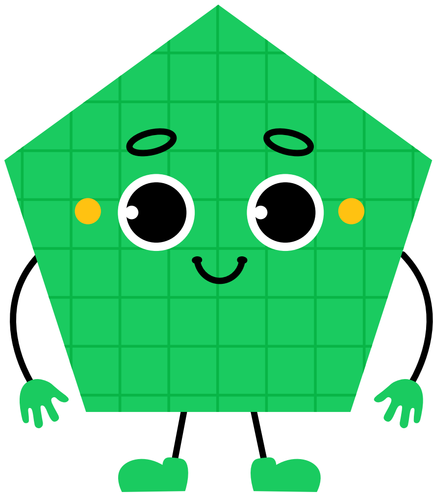
pentagon
